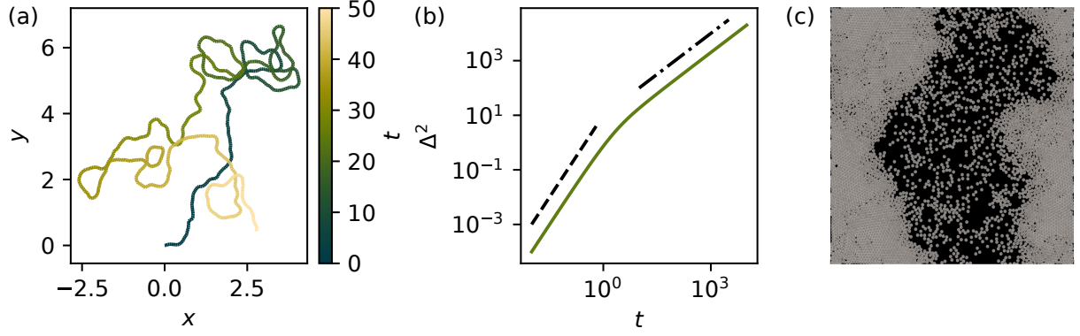
Figure 2.4: (a) Typical trajectory of an active Brownian particle ( U = D_r = 1 ). (b) Mean square displacement \Delta^2 from Eq. (2.107). The two black lines show the slopes 2 and 1 corresponding to the limits of short and large times. (c) Motility-induced phase separation ( U = 100, D_r = 1 , simulations: Nikita Allaglo). At high activity an assembly of ABPs separate into a dense cluster and a dilute phase.
